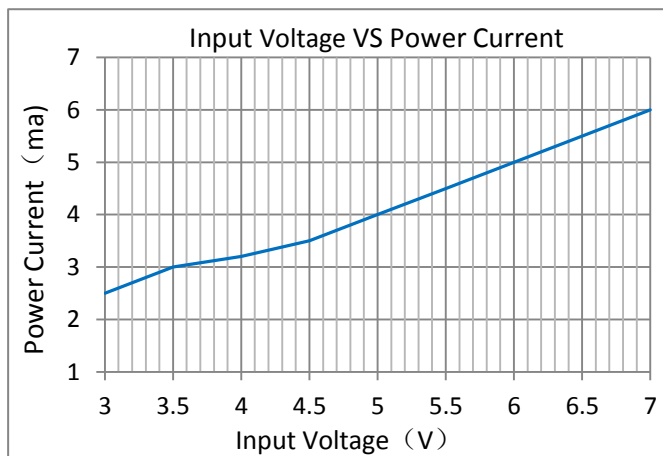
图6: Power Crrent VS. Supply Voltage
